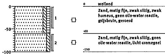
Boring: 03
