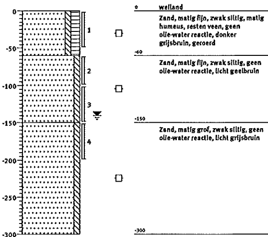
Boring: 06
