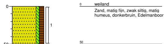
Boring: A04
