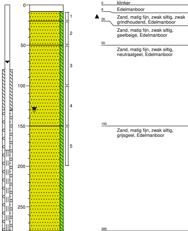
Boring: A01
