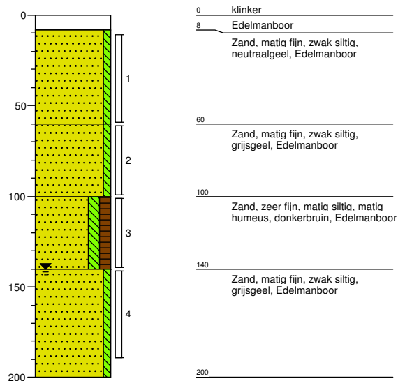
Boring: A03
