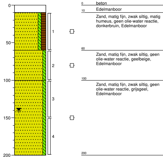
Boring: B02
