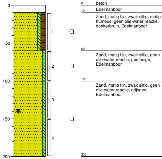
Boring: B01
