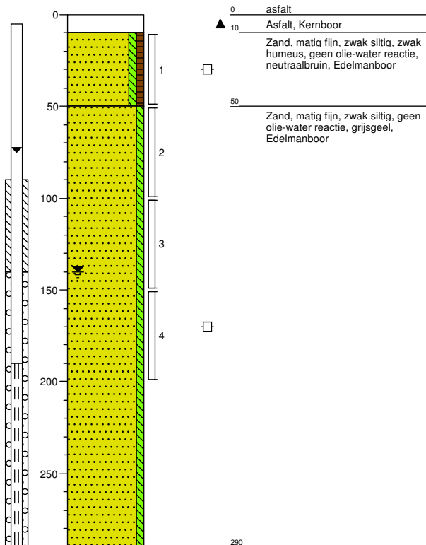
Boring: B03
