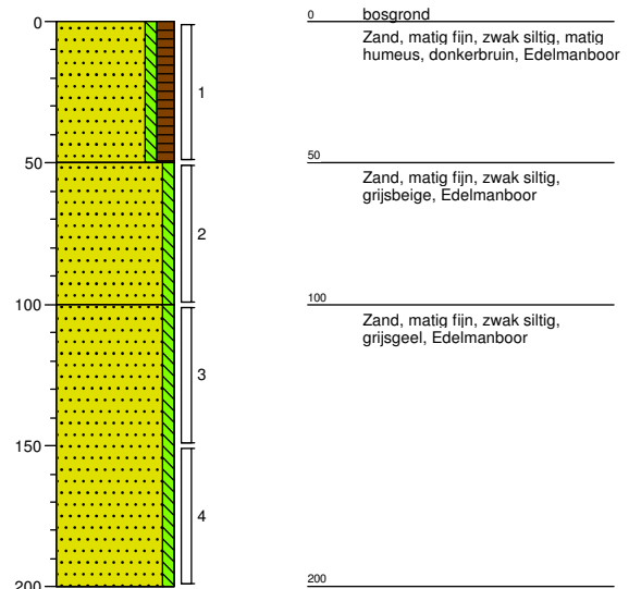
Boring: A02
