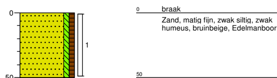
Boring: A05
