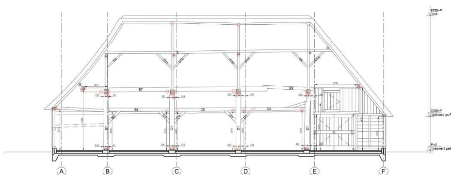
LANGSDOORSNEDE as 2
