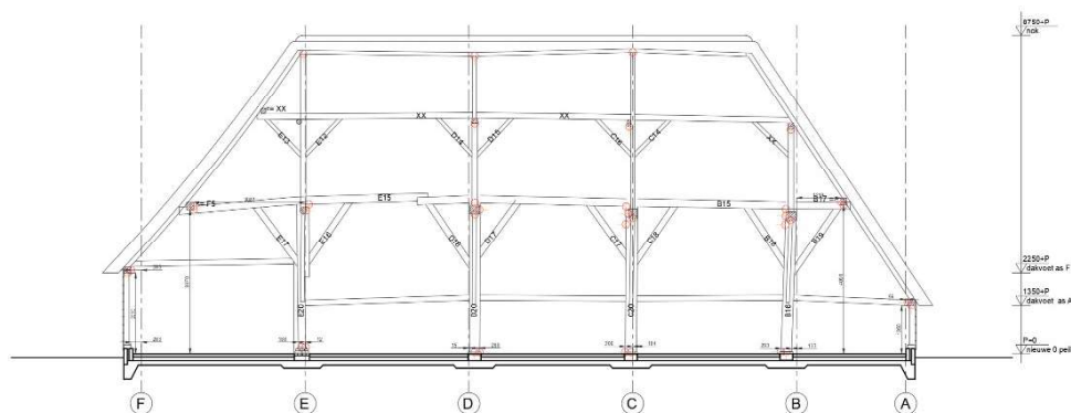
LANGSDOORSNEDE as 4
