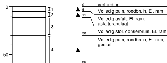
Boring: 04
