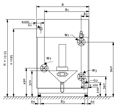
Fig. 43 Afmetingen R2900SB split system
