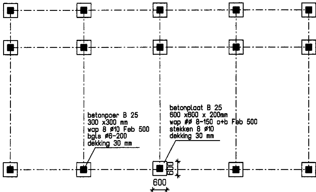
Fundering
