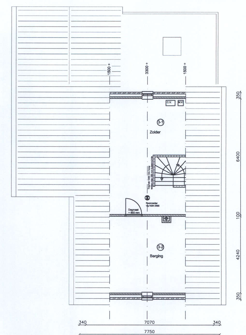
Zolder
