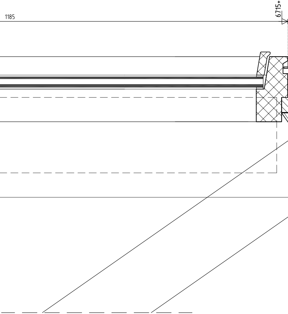
DETAIL 3
