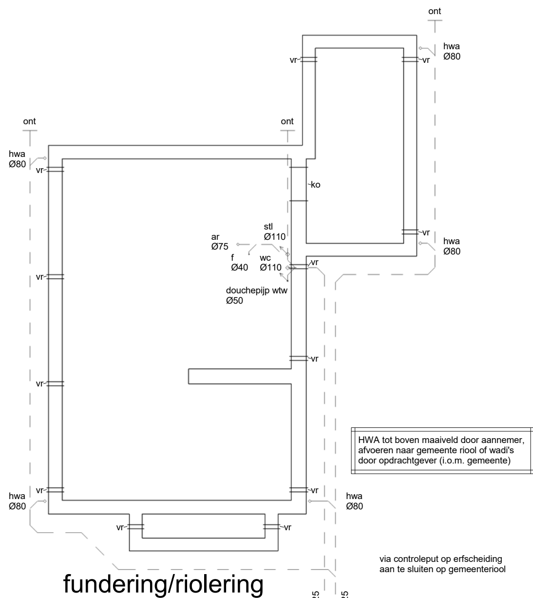
fundering/riolering
