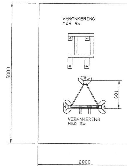
FUNDERING
