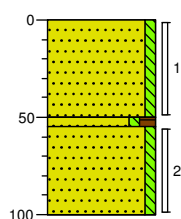
Boring: 03
