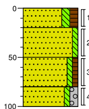
Boring: 14
