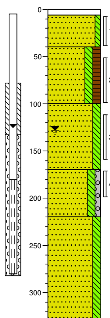
Boring: 06
