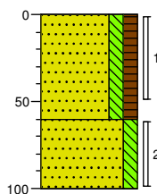
Boring: 08
