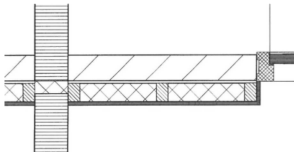
DETAIL 5
