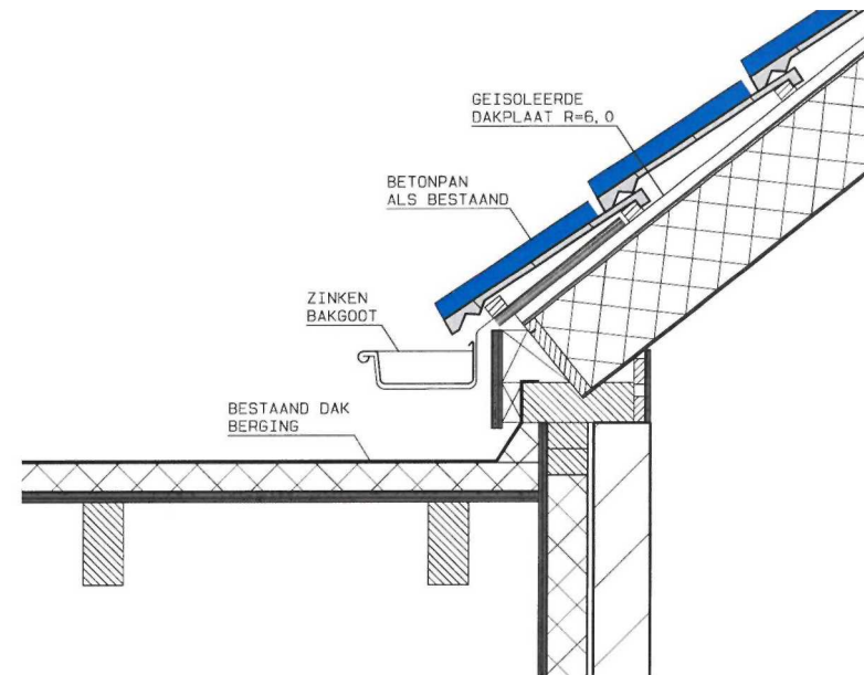
DETAIL 7
