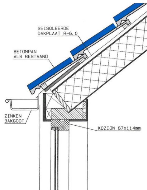
DETAIL 6
