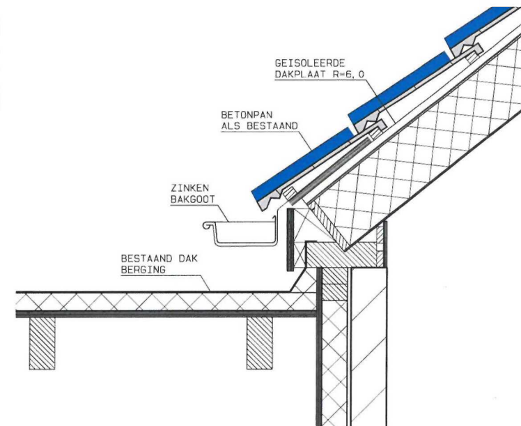
DETAIL 7
