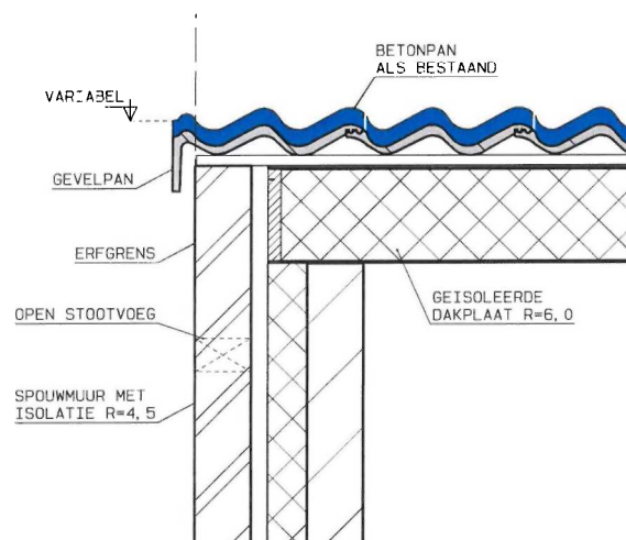
DETAIL 4
