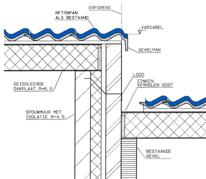
DETAIL 4
